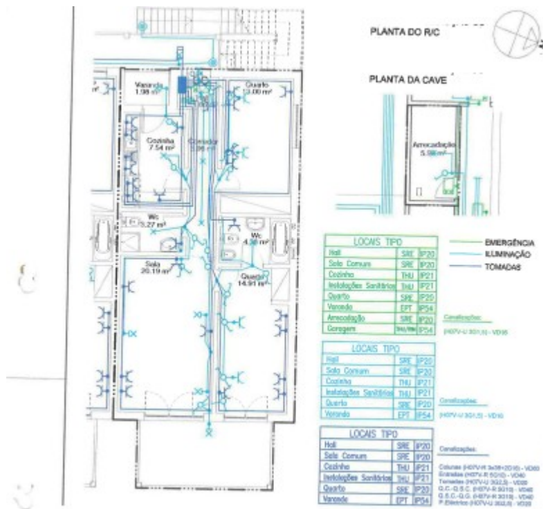
LG2233 Floor plans
