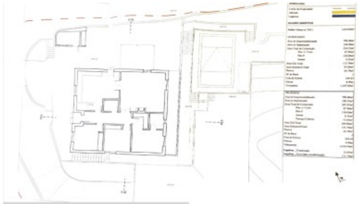
Floor plan 1
