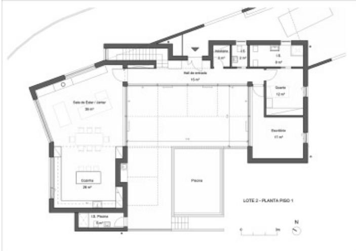
Floorplan Lote 2
